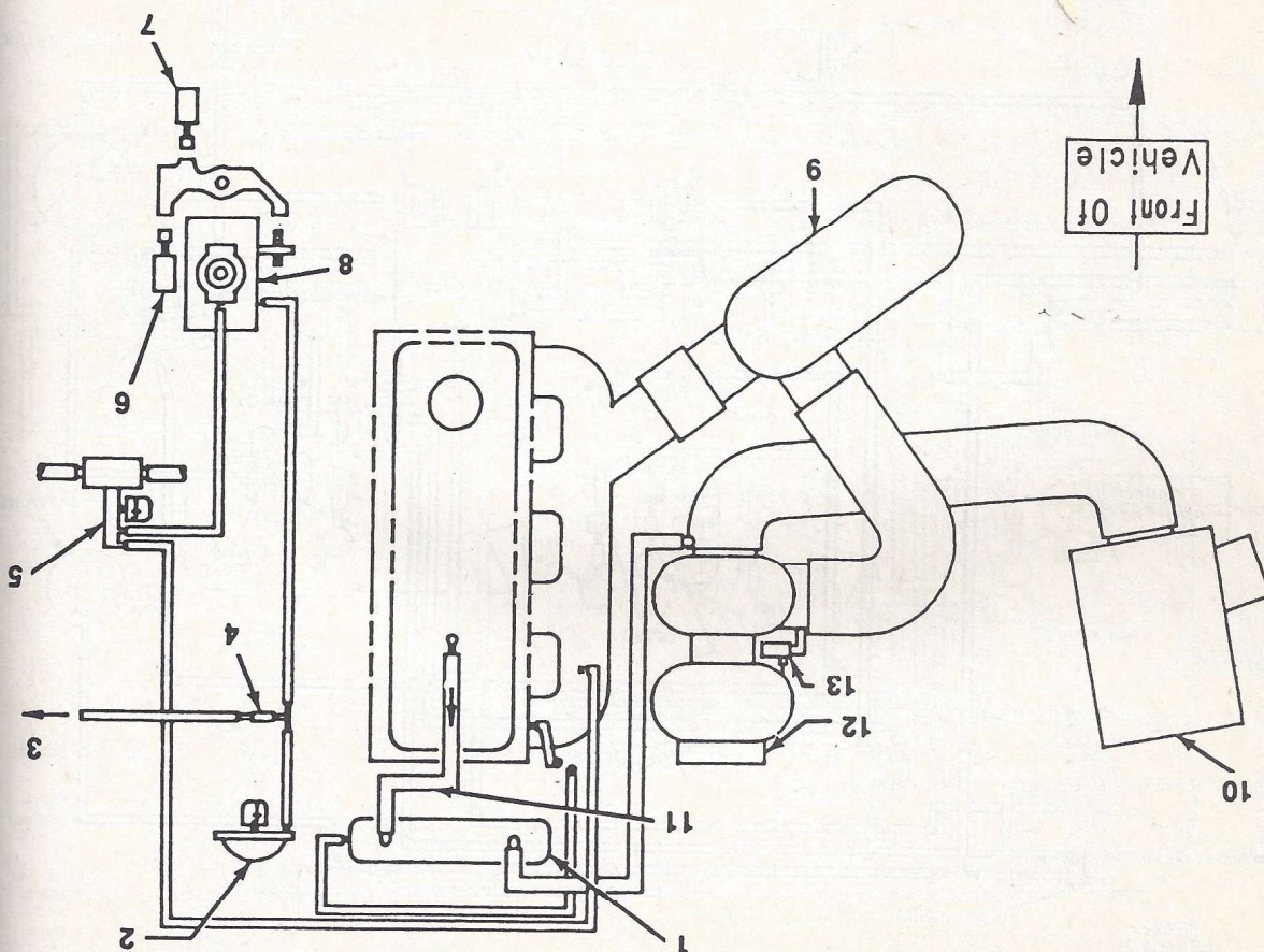
DIESEL ENGINE VACUUM ROUTING
